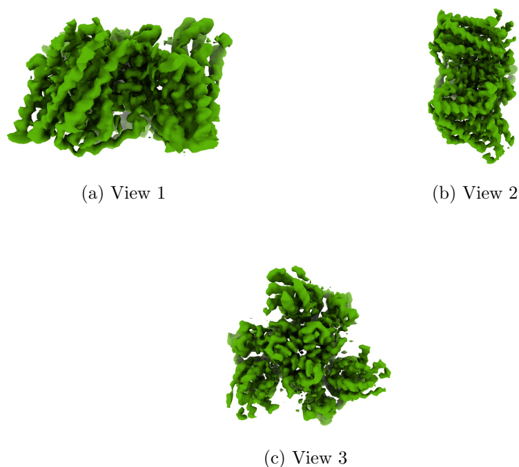
Figure 4: Isosurface at threshold=0.348000. Views generated by ChimeraX at a the following X, Y, Z angles: View 1 (0, -90, -90), View 2 (-90, 0, -90), View 3 (0, 0, 0).
