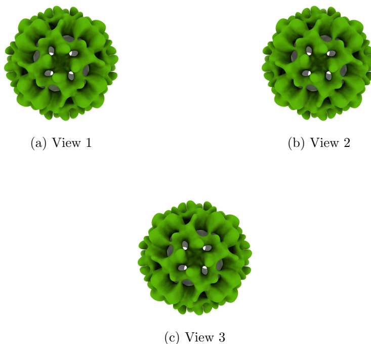
Figure 4: Isosurface at threshold=0.215000. Views generated by ChimeraX at a the following X, Y, Z angles: View 1 (0, -90, -90), View 2 (-90, 0, -90), View 3 (0, 0, 0).
