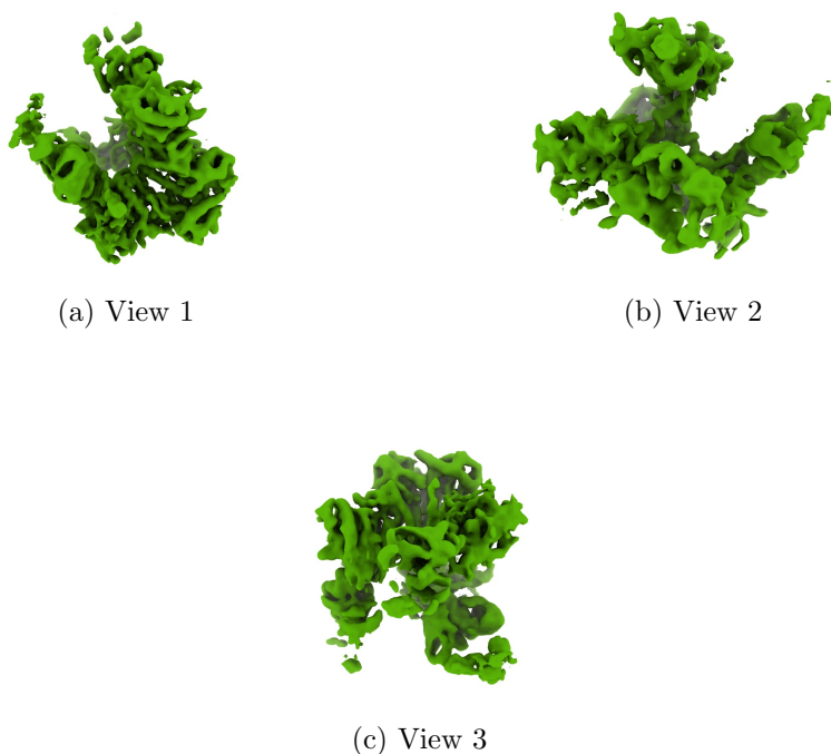
Figure 4: Isosurface at threshold=0.081600. Views generated by ChimeraX at a the following X, Y, Z angles: View 1 (0, -90, -90), View 2 (-90, 0, -90), View 3 (0, 0, 0).
