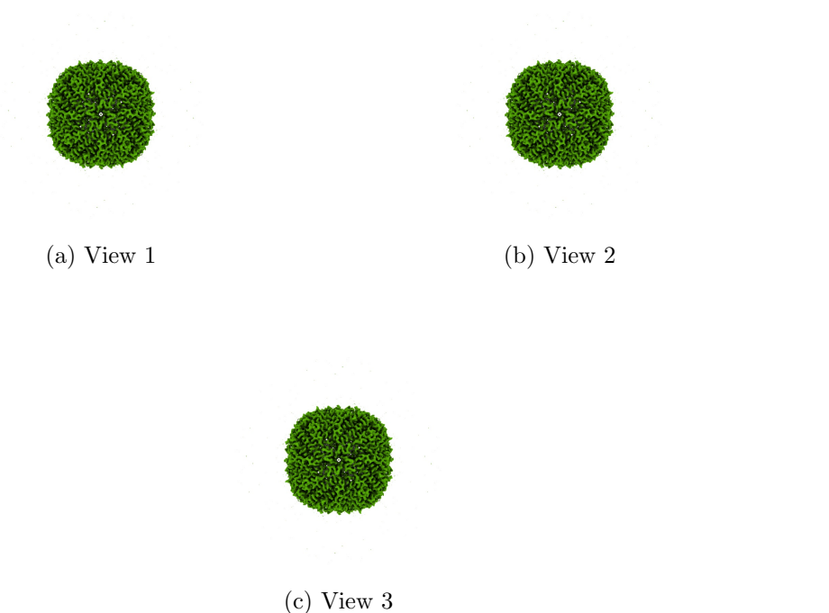
Figure 4: Isosurface at threshold=0.600000. Views generated by ChimeraX at a the following X, Y, Z angles: View 1 (0, -90, -90), View 2 (-90, 0, -90), View 3 (0, 0, 0).
