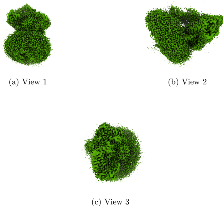
Figure 4: Isosurface at threshold=0.181000. Views generated by ChimeraX at a the following X, Y, Z angles: View 1 (0, -90, -90), View 2 (-90, 0, -90), View 3 (0, 0, 0).
