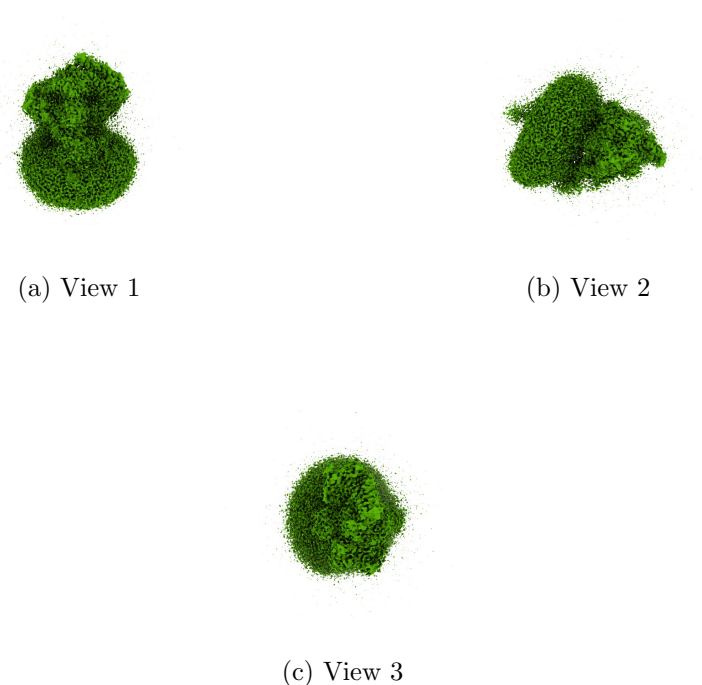
Figure 4: Isosurface at threshold=0.185000. Views generated by ChimeraX at a the following X, Y, Z angles: View 1 (0, -90, -90), View 2 (-90, 0, -90), View 3 (0, 0, 0).
