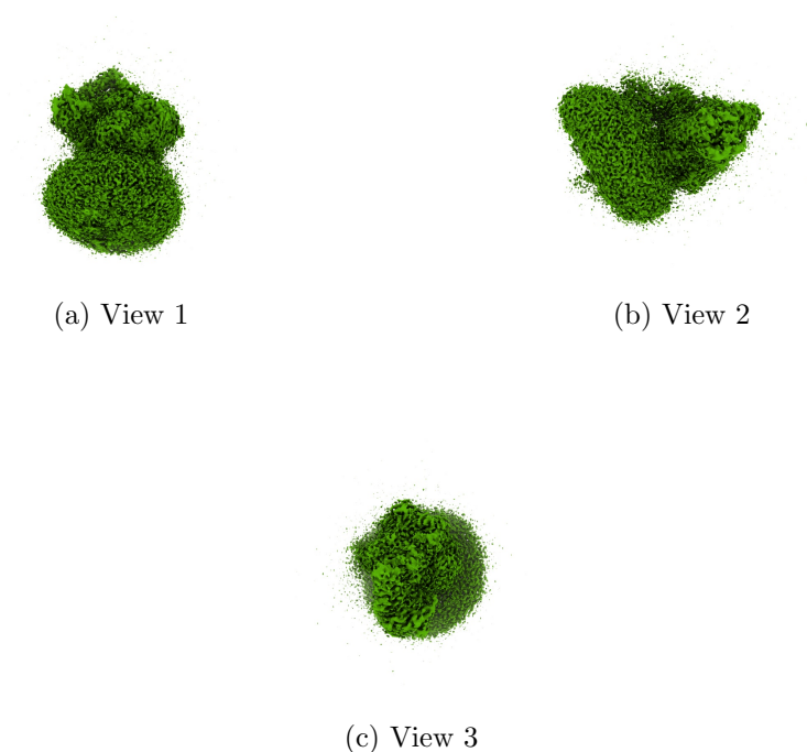
Figure 4: Isosurface at threshold=0.183000. Views generated by ChimeraX at a the following X, Y, Z angles: View 1 (0, -90, -90), View 2 (-90, 0, -90), View 3 (0, 0, 0).
