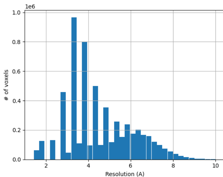
Figure 29: Histogram of the local resolution according to MonoRes.
