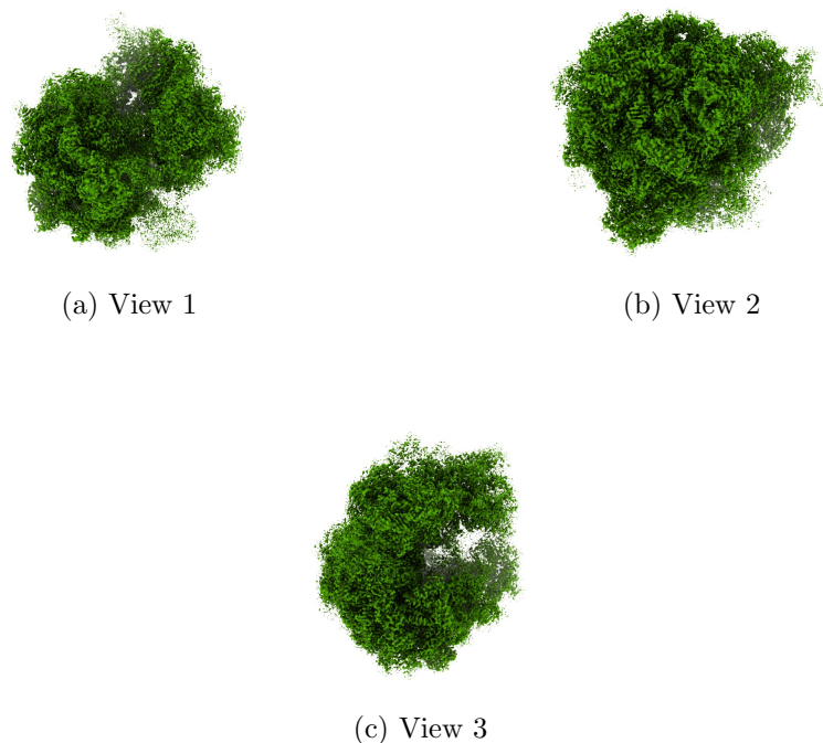
Figure 4: Isosurface at threshold=0.030600. Views generated by ChimeraX at a the following X, Y, Z angles: View 1 (0, -90, -90), View 2 (-90, 0, -90), View 3 (0, 0, 0).
