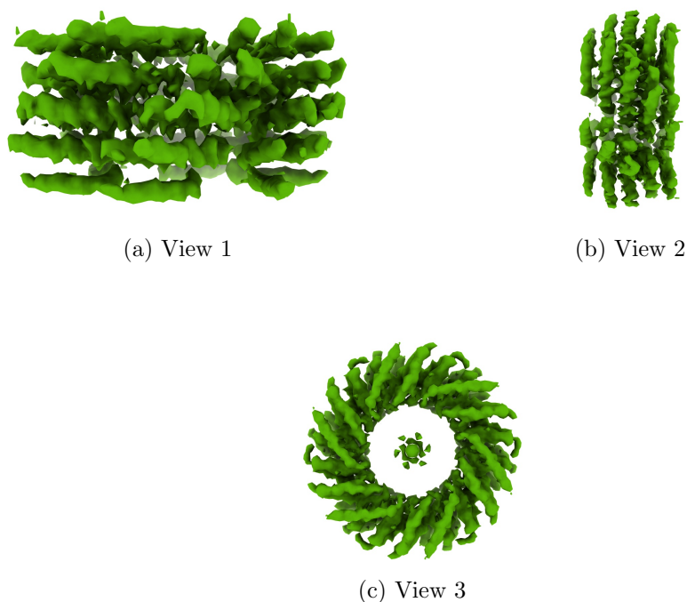
Figure 4: Isosurface at threshold=0.207000. Views generated by ChimeraX at a the following X, Y, Z angles: View 1 (0, -90, -90), View 2 (-90, 0, -90), View 3 (0, 0, 0).
