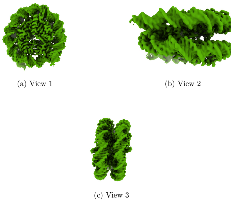
Figure 4: Isosurface at threshold=0.054000. Views generated by ChimeraX at a the following X, Y, Z angles: View 1 (0, -90, -90), View 2 (-90, 0, -90), View 3 (0, 0, 0).
