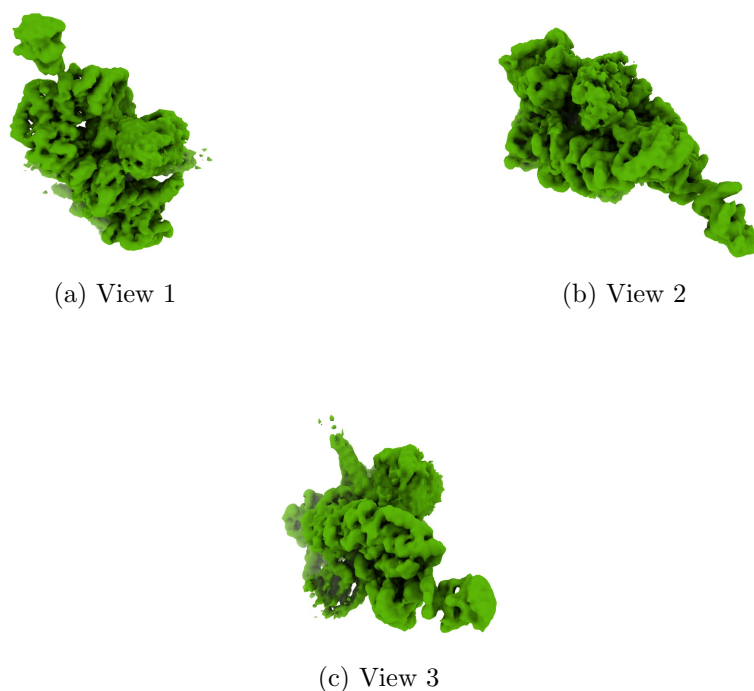
Figure 4: Isosurface at threshold=0.006110. Views generated by ChimeraX at a the following X, Y, Z angles: View 1 (0, -90, -90), View 2 (-90, 0, -90), View 3 (0, 0, 0).
