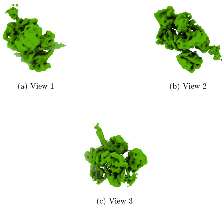
Figure 4: Isosurface at threshold=0.003680. Views generated by ChimeraX at a the following X, Y, Z angles: View 1 (0, -90, -90), View 2 (-90, 0, -90), View 3 (0, 0, 0).
