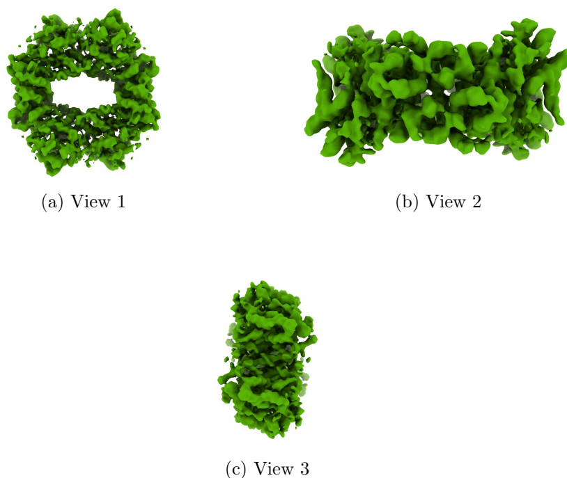
Figure 4: Isosurface at threshold=2.500000. Views generated by ChimeraX at the following X, Y, Z angles: View 1 (0, -90, -90), View 2 (-90, 0, -90), View 3 (0, 0, 0).
