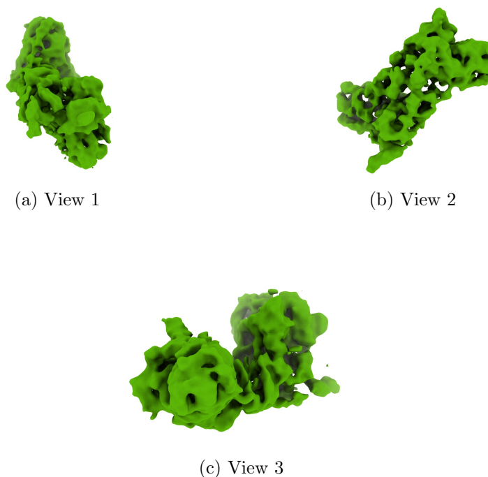
Figure 4: Isosurface at threshold=2.000000. Views generated by ChimeraX at a the following X, Y, Z angles: View 1 (0, -90, -90), View 2 (-90, 0, -90), View 3 (0, 0, 0).
