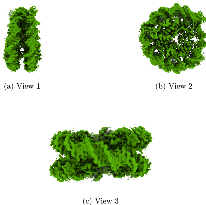
Figure 4: Isosurface at threshold=4.750000. Views generated by ChimeraX at a the following X, Y, Z angles: View 1 (0, -90, -90), View 2 (-90, 0, -90), View 3 (0, 0, 0).
