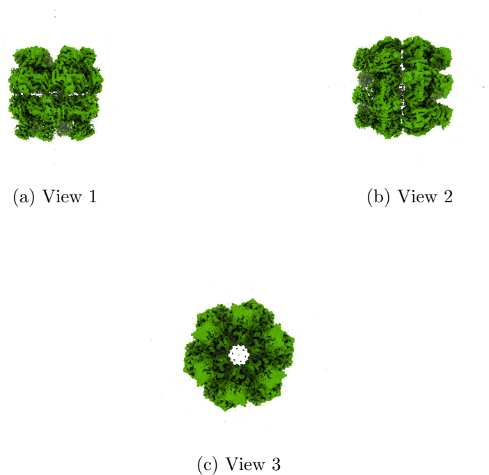
Figure 4: Isosurface at threshold=0.056100. Views generated by ChimeraX at a the following X, Y, Z angles: View 1 (0, -90, -90), View 2 (-90, 0, -90), View 3 (0, 0, 0).
