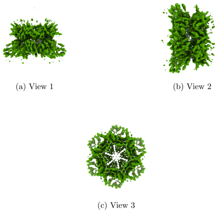
Figure 4: Isosurface at threshold=0.282000. Views generated by ChimeraX at a the following X, Y, Z angles: View 1 (0, -90, -90), View 2 (-90, 0, -90), View 3 (0, 0, 0).
