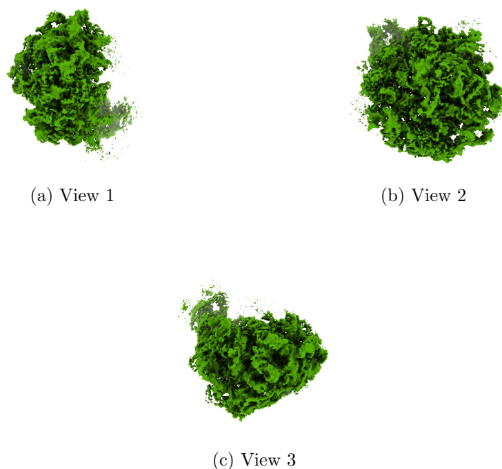
Figure 4: Isosurface at threshold=0.046000. Views generated by ChimeraX at a the following X, Y, Z angles: View 1 (0, -90, -90), View 2 (-90, 0, -90), View 3 (0, 0, 0).
