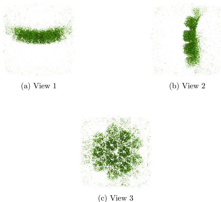
Figure 4: Isosurface at threshold=9.440000. Views generated by ChimeraX at a the following X, Y, Z angles: View 1 (0, -90, -90), View 2 (-90, 0, -90), View 3 (0, 0, 0).
