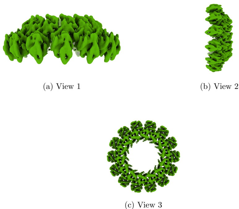
Figure 4: Isosurface at threshold=0.001900. Views generated by ChimeraX at a the following X, Y, Z angles: View 1 (0, -90, -90), View 2 (-90, 0, -90), View 3 (0, 0, 0).
