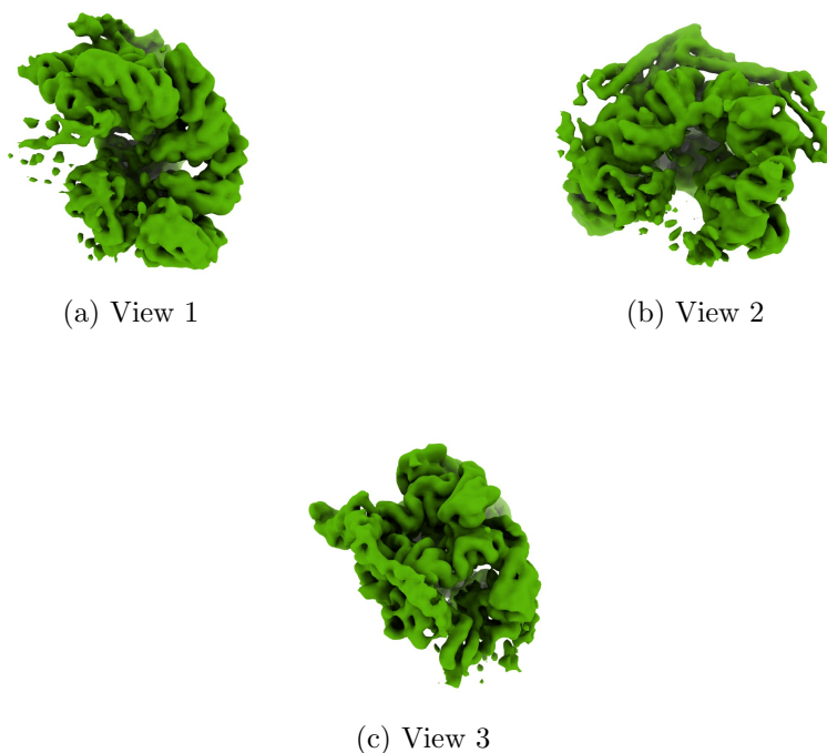
Figure 4: Isosurface at threshold=0.009200. Views generated by ChimeraX at a the following X, Y, Z angles: View 1 (0, -90, -90), View 2 (-90, 0, -90), View 3 (0, 0, 0).
