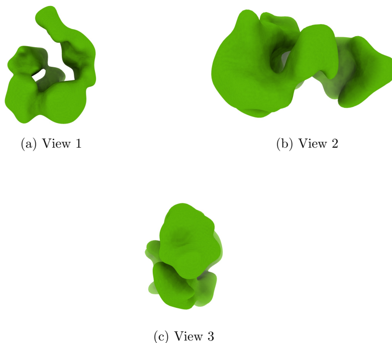
Figure 4: Isosurface at threshold=0.042500. Views generated by ChimeraX at a the following X, Y, Z angles: View 1 (0, -90, -90), View 2 (-90, 0, -90), View 3 (0, 0, 0).
