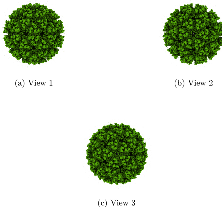
Figure 4: Isosurface at threshold=1.800000. Views generated by ChimeraX at a the following X, Y, Z angles: View 1 (0, -90, -90), View 2 (-90, 0, -90), View 3 (0, 0, 0).
