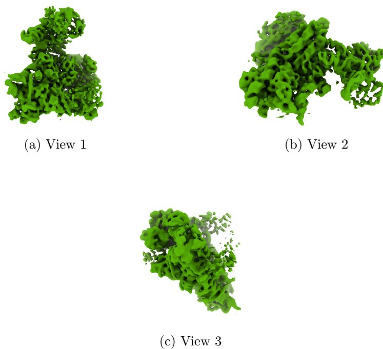
Figure 4: Isosurface at threshold=0.096600. Views generated by ChimeraX at a the following X, Y, Z angles: View 1 (0, -90, -90), View 2 (-90, 0, -90), View 3 (0, 0, 0).
