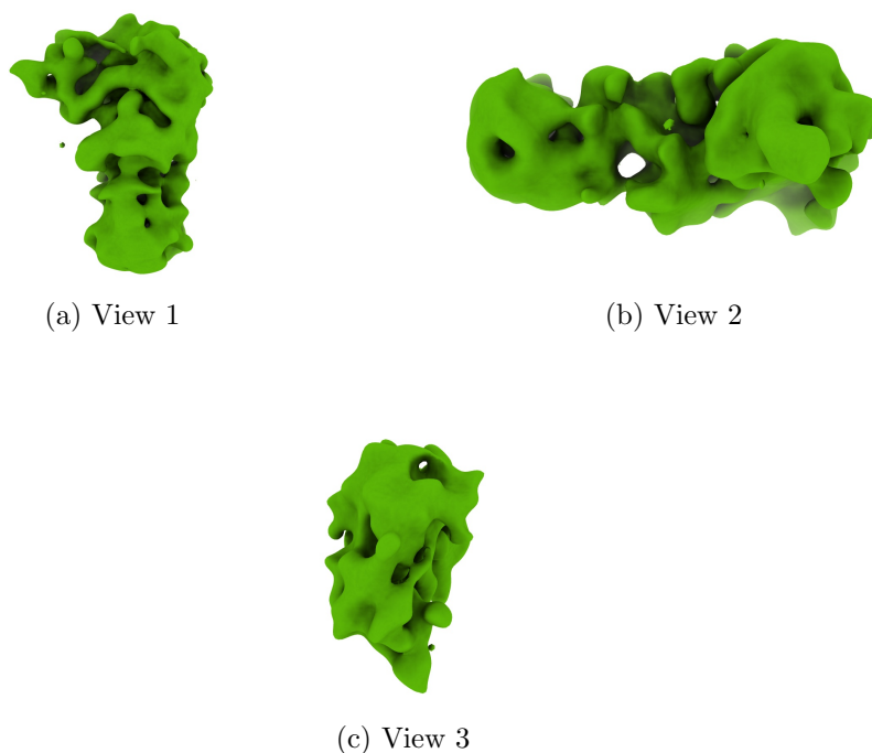
Figure 4: Isosurface at threshold=0.004100. Views generated by ChimeraX at a the following X, Y, Z angles: View 1 (0, -90, -90), View 2 (-90, 0, -90), View 3 (0, 0, 0).
