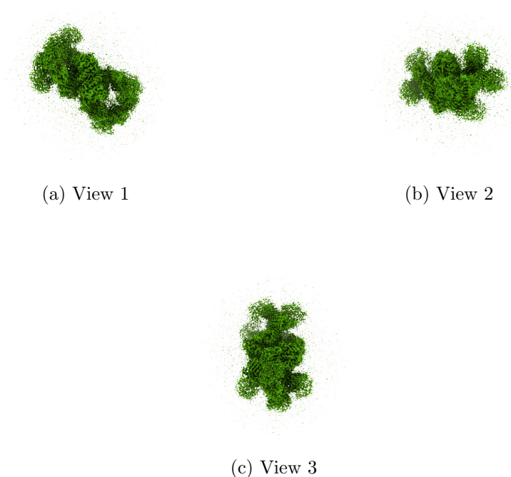
Figure 4: Isosurface at threshold=0.038900. Views generated by ChimeraX at a the following X, Y, Z angles: View 1 (0, -90, -90), View 2 (-90, 0, -90), View 3 (0, 0, 0).
