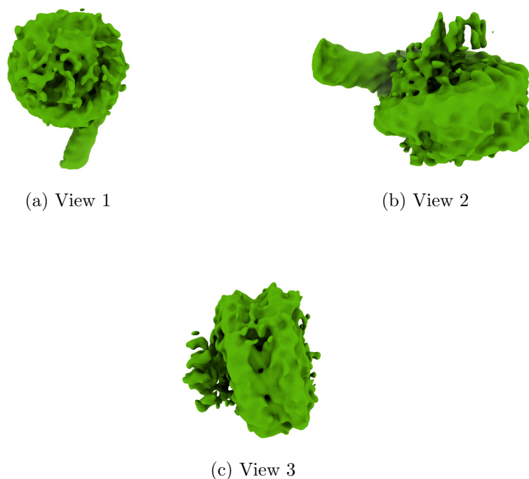
Figure 4: Isosurface at threshold=0.006270. Views generated by ChimeraX at a the following X, Y, Z angles: View 1 (0, -90, -90), View 2 (-90, 0, -90), View 3 (0, 0, 0).
