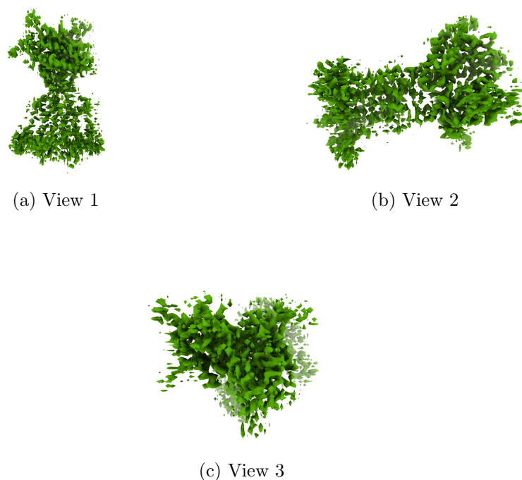
Figure 4: Isosurface at threshold=0.073600. Views generated by ChimeraX at the following X, Y, Z angles: View 1 (0, -90, -90), View 2 (-90, 0, -90), View 3 (0, 0, 0).
