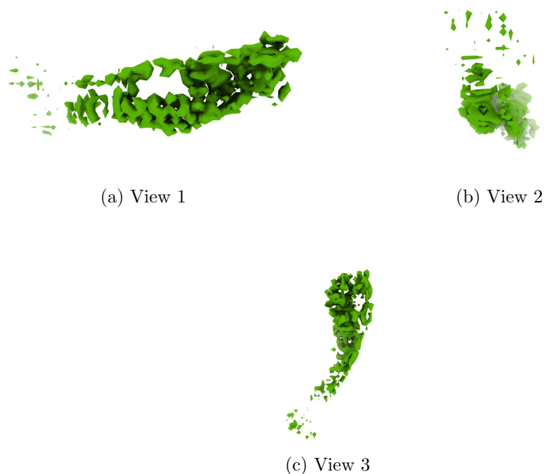
Figure 4: Isosurface at threshold=0.018000. Views generated by ChimeraX at a the following X, Y, Z angles: View 1 (0, -90, -90), View 2 (-90, 0, -90), View 3 (0, 0, 0).
