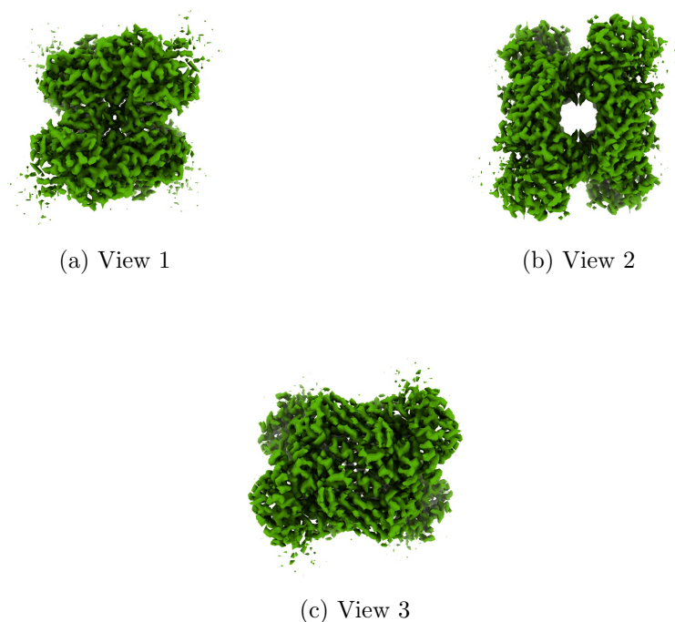
Figure 4: Isosurface at threshold=0.042000. Views generated by ChimeraX at a the following X, Y, Z angles: View 1 (0, -90, -90), View 2 (-90, 0, -90), View 3 (0, 0, 0).
