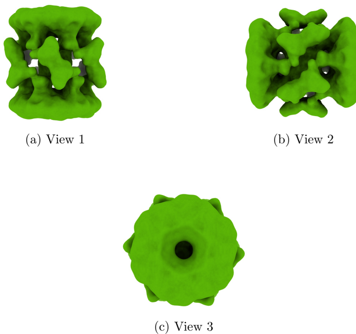
Figure 4: Isosurface at threshold=2.410000. Views generated by ChimeraX at a the following X, Y, Z angles: View 1 (0, -90, -90), View 2 (-90, 0, -90), View 3 (0, 0, 0).
