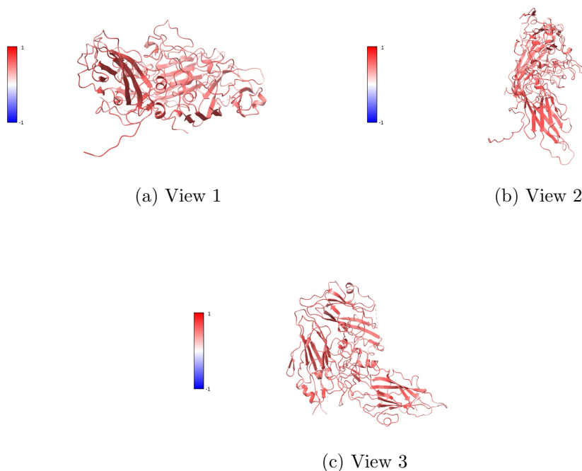
Figure 17: Atomic model colored by MapQ Views generated by ChimeraX at the following X, Y, Z angles: View 1 (0, -90, -90), View 2 (-90, 0, -90), View 3 (0, 0, 0).
