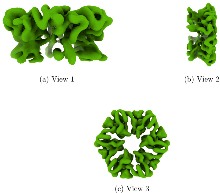
Figure 4: Isosurface at threshold=0.032500. Views generated by ChimeraX at a the following X, Y, Z angles: View 1 (0, -90, -90), View 2 (-90, 0, -90), View 3 (0, 0, 0).
