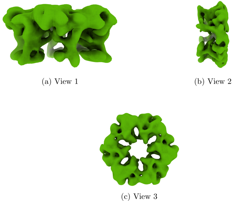
Figure 4: Isosurface at threshold=0.026200. Views generated by ChimeraX at a the following X, Y, Z angles: View 1 (0, -90, -90), View 2 (-90, 0, -90), View 3 (0, 0, 0).
