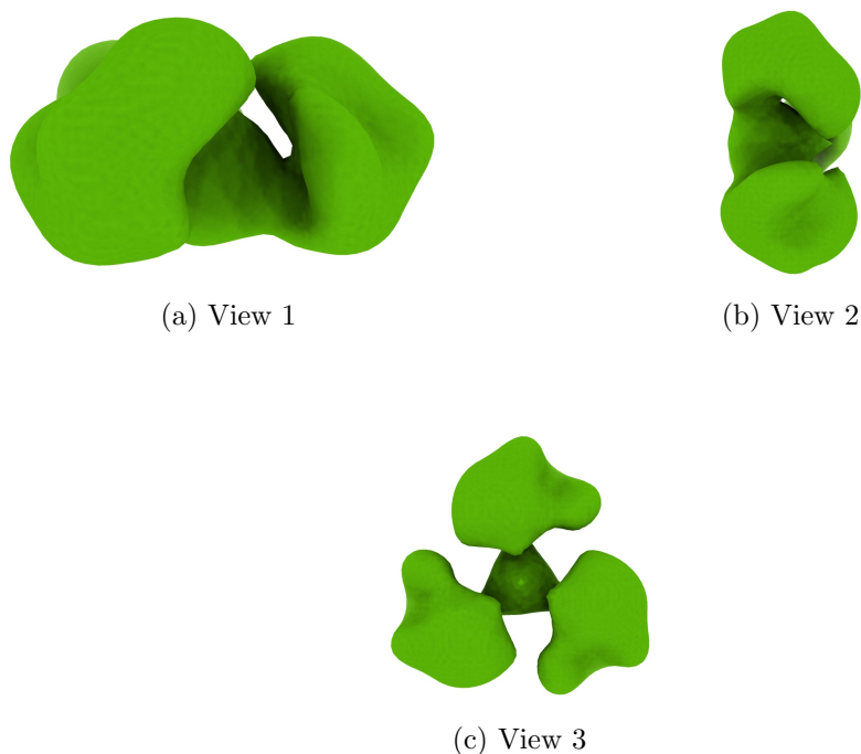
Figure 4: Isosurface at threshold=0.089800. Views generated by ChimeraX at a the following X, Y, Z angles: View 1 (0, -90, -90), View 2 (-90, 0, -90), View 3 (0, 0, 0).
