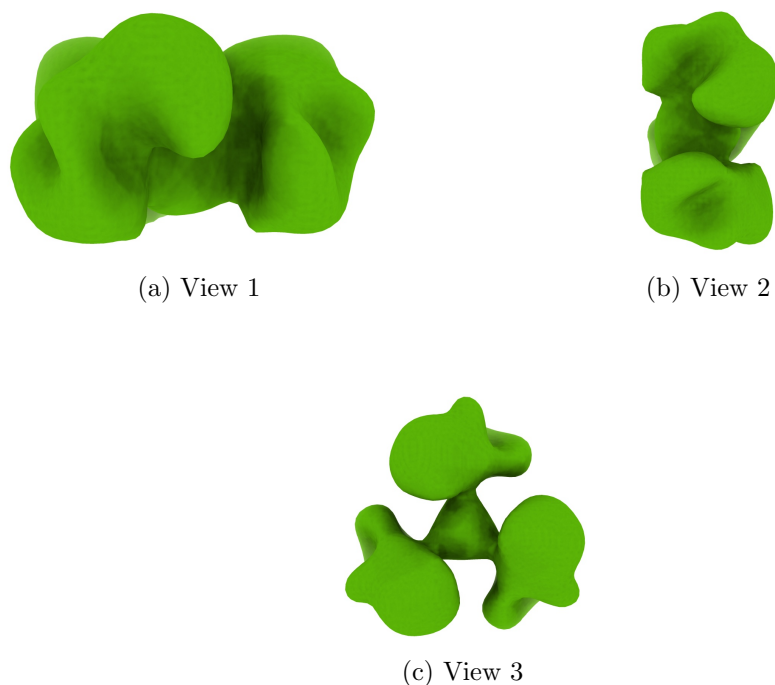
Figure 4: Isosurface at threshold=0.095800. Views generated by ChimeraX at a the following X, Y, Z angles: View 1 (0, -90, -90), View 2 (-90, 0, -90), View 3 (0, 0, 0).
