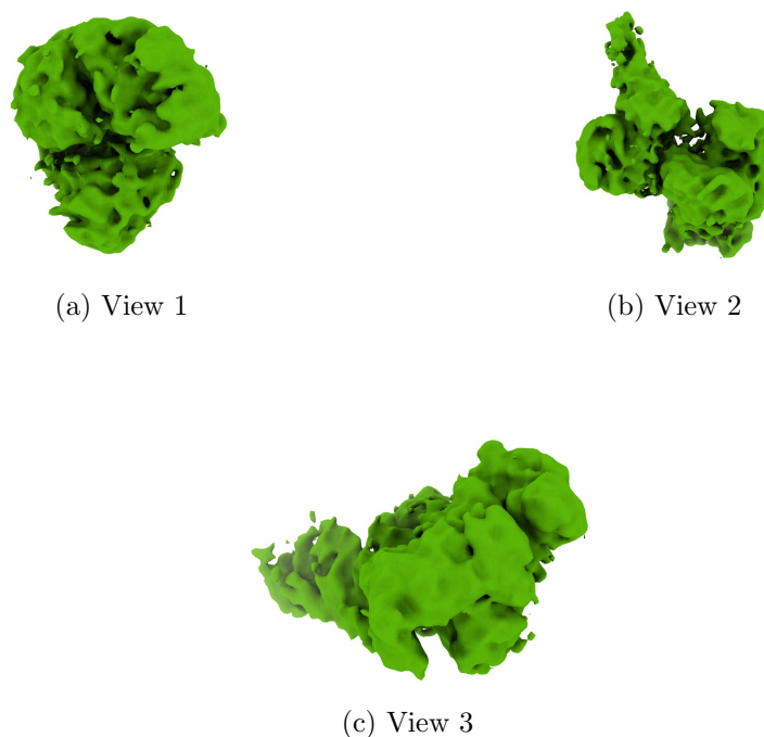
Figure 4: Isosurface at threshold=0.006640. Views generated by ChimeraX at a the following X, Y, Z angles: View 1 (0, -90, -90), View 2 (-90, 0, -90), View 3 (0, 0, 0).
