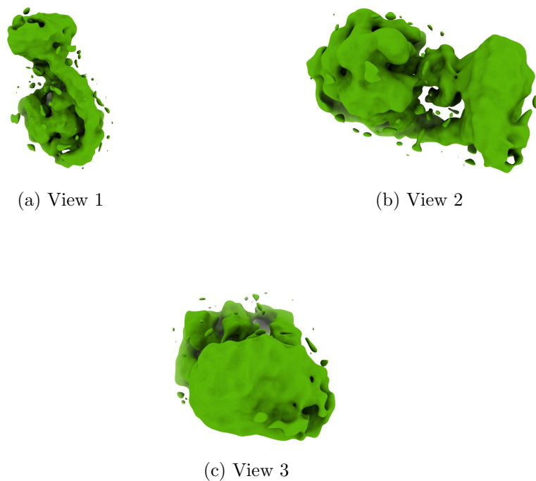
Figure 4: Isosurface at threshold=31.000000. Views generated by ChimeraX at a the following X, Y, Z angles: View 1 (0, -90, -90), View 2 (-90, 0, -90), View 3 (0, 0, 0).
