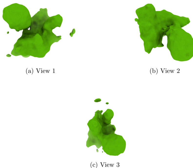
Figure 4: Isosurface at threshold=4.580000. Views generated by ChimeraX at a the following X, Y, Z angles: View 1 (0, -90, -90), View 2 (-90, 0, -90), View 3 (0, 0, 0).
