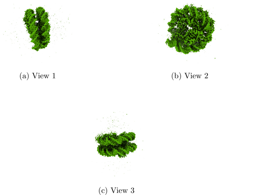
Figure 4: Isosurface at threshold=0.018600. Views generated by ChimeraX at a the following X, Y, Z angles: View 1 (0, -90, -90), View 2 (-90, 0, -90), View 3 (0, 0, 0).
