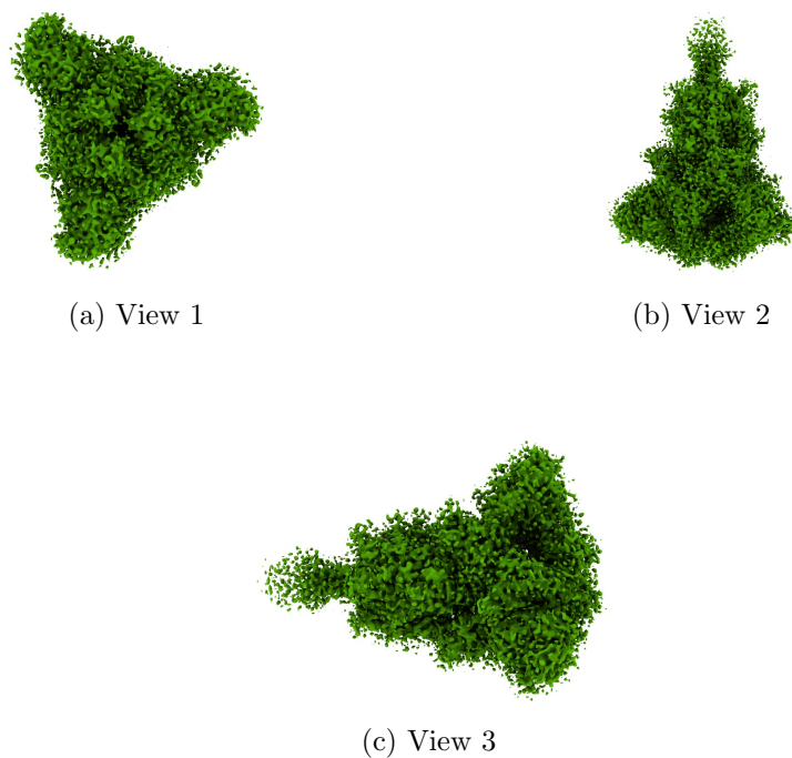
Figure 4: Isosurface at threshold=2.980000. Views generated by ChimeraX at a the following X, Y, Z angles: View 1 (0, -90, -90), View 2 (-90, 0, -90), View 3 (0, 0, 0).
