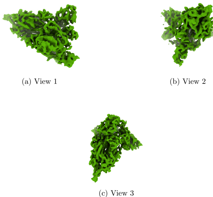
Figure 4: Isosurface at threshold=0.014300. Views generated by ChimeraX at the following X, Y, Z angles: View 1 (0, -90, -90), View 2 (-90, 0, -90), View 3 (0, 0, 0).
