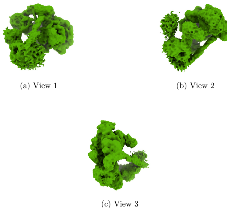
Figure 4: Isosurface at threshold=0.180000. Views generated by ChimeraX at the following X, Y, Z angles: View 1 (0, -90, -90), View 2 (-90, 0, -90), View 3 (0, 0, 0).
