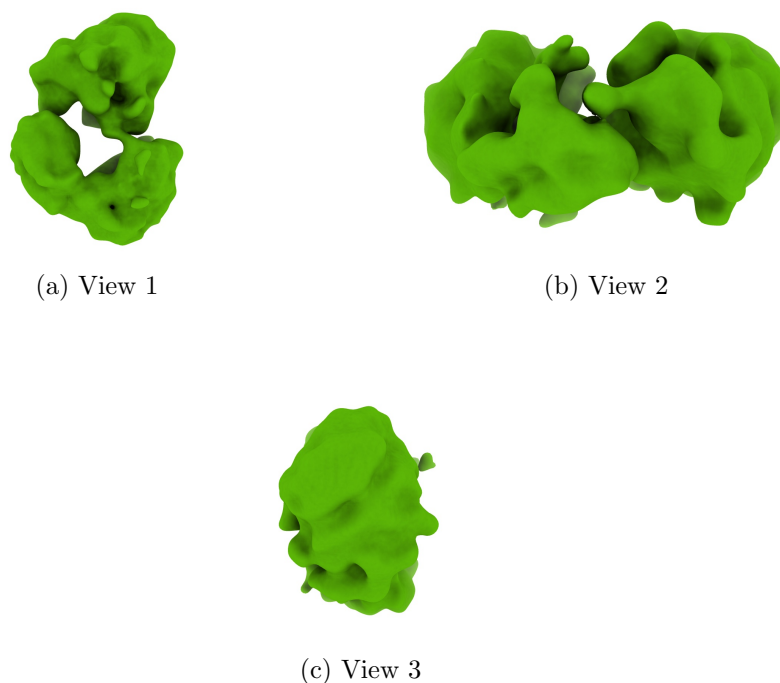
Figure 4: Isosurface at threshold=0.277000. Views generated by ChimeraX at a the following X, Y, Z angles: View 1 (0, -90, -90), View 2 (-90, 0, -90), View 3 (0, 0, 0).
