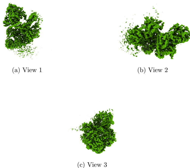
Figure 4: Isosurface at threshold=0.560000. Views generated by ChimeraX at a the following X, Y, Z angles: View 1 (0, -90, -90), View 2 (-90, 0, -90), View 3 (0, 0, 0).
