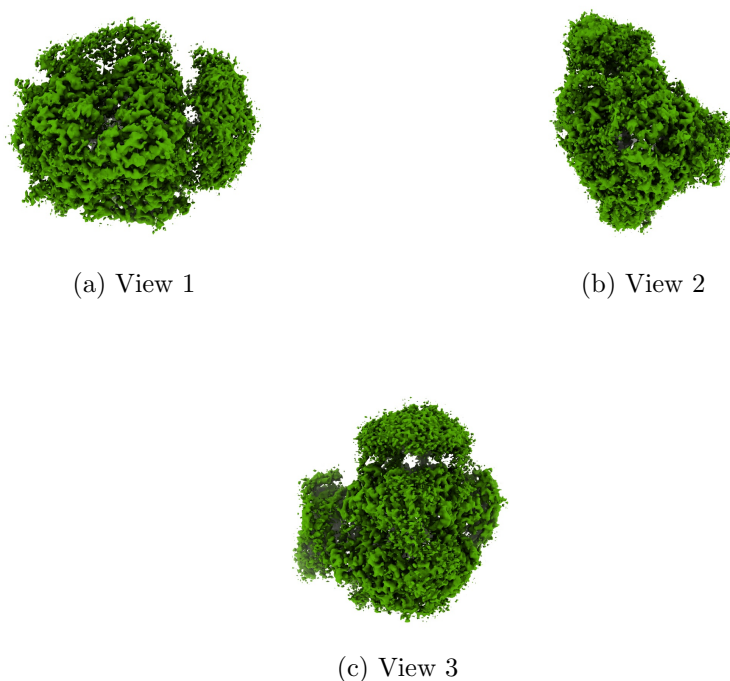
Figure 4: Isosurface at threshold=0.852000. Views generated by ChimeraX at a the following X, Y, Z angles: View 1 (0, -90, -90), View 2 (-90, 0, -90), View 3 (0, 0, 0).
