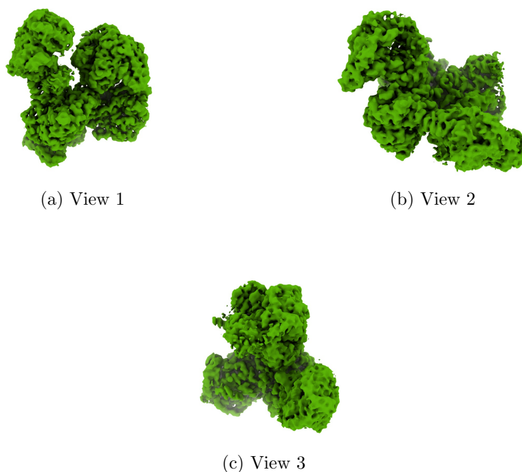
Figure 4: Isosurface at threshold=0.008500. Views generated by ChimeraX at the following X, Y, Z angles: View 1 (0, -90, -90), View 2 (-90, 0, -90), View 3 (0, 0, 0).
