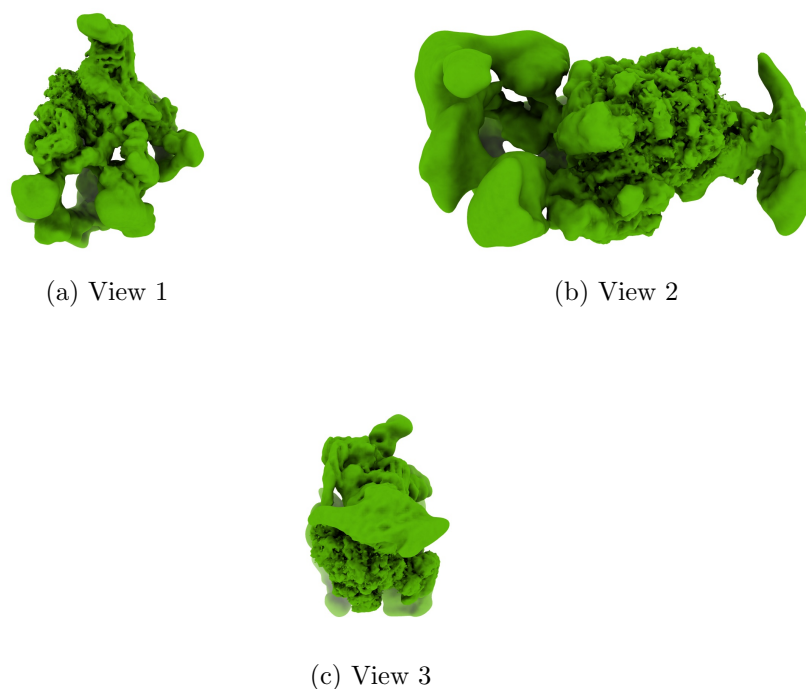
Figure 4: Isosurface at threshold=0.490000. Views generated by ChimeraX at a the following X, Y, Z angles: View 1 (0, -90, -90), View 2 (-90, 0, -90), View 3 (0, 0, 0).
