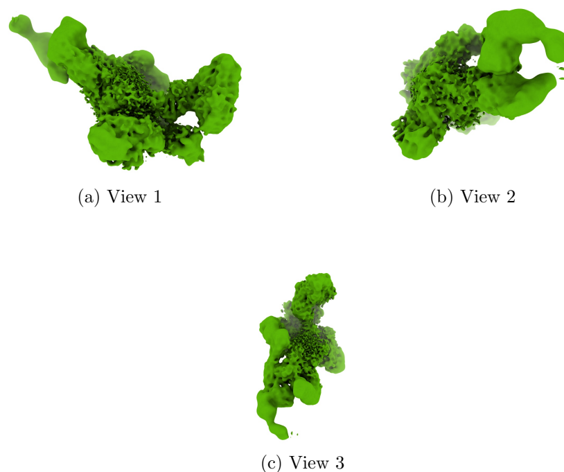
Figure 4: Isosurface at threshold=0.600000. Views generated by ChimeraX at a the following X, Y, Z angles: View 1 (0, -90, -90), View 2 (-90, 0, -90), View 3 (0, 0, 0).
